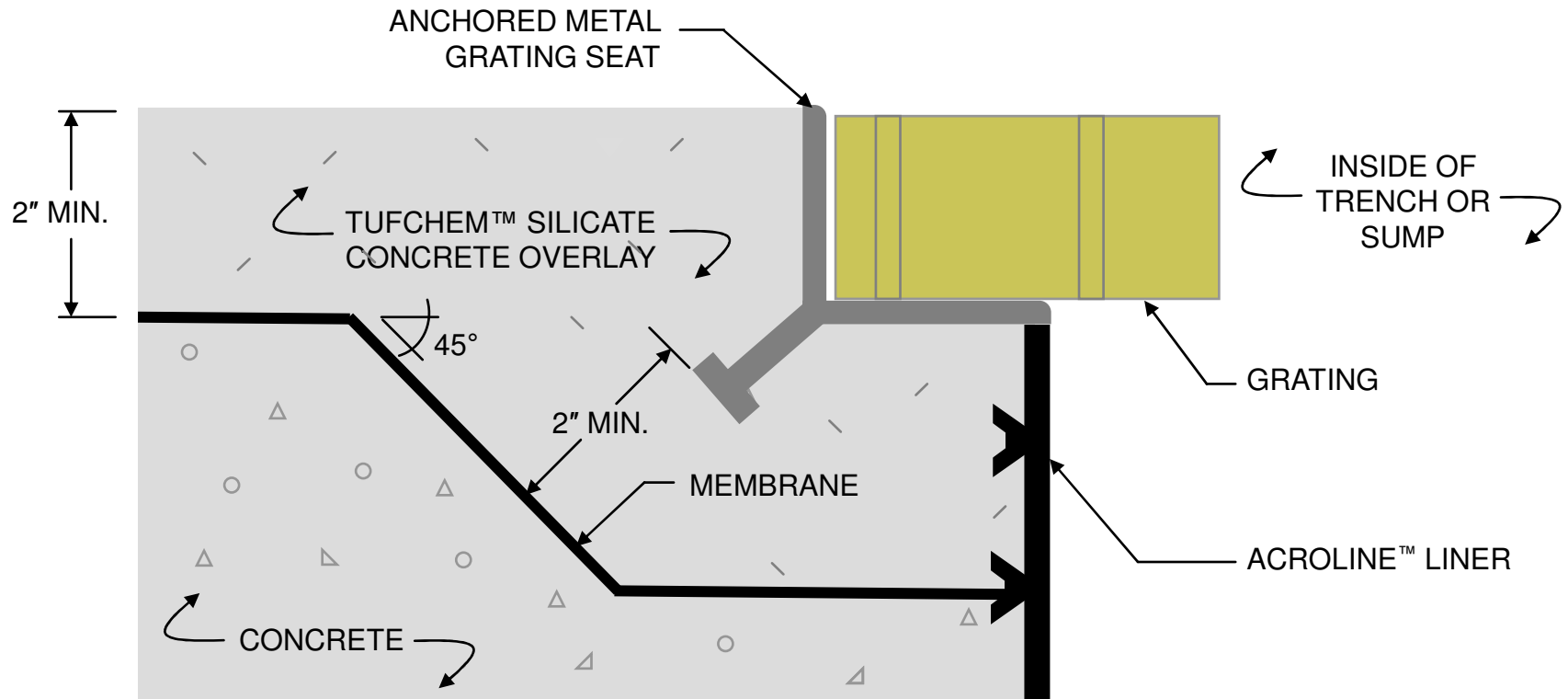
ELEVATION VIEW
